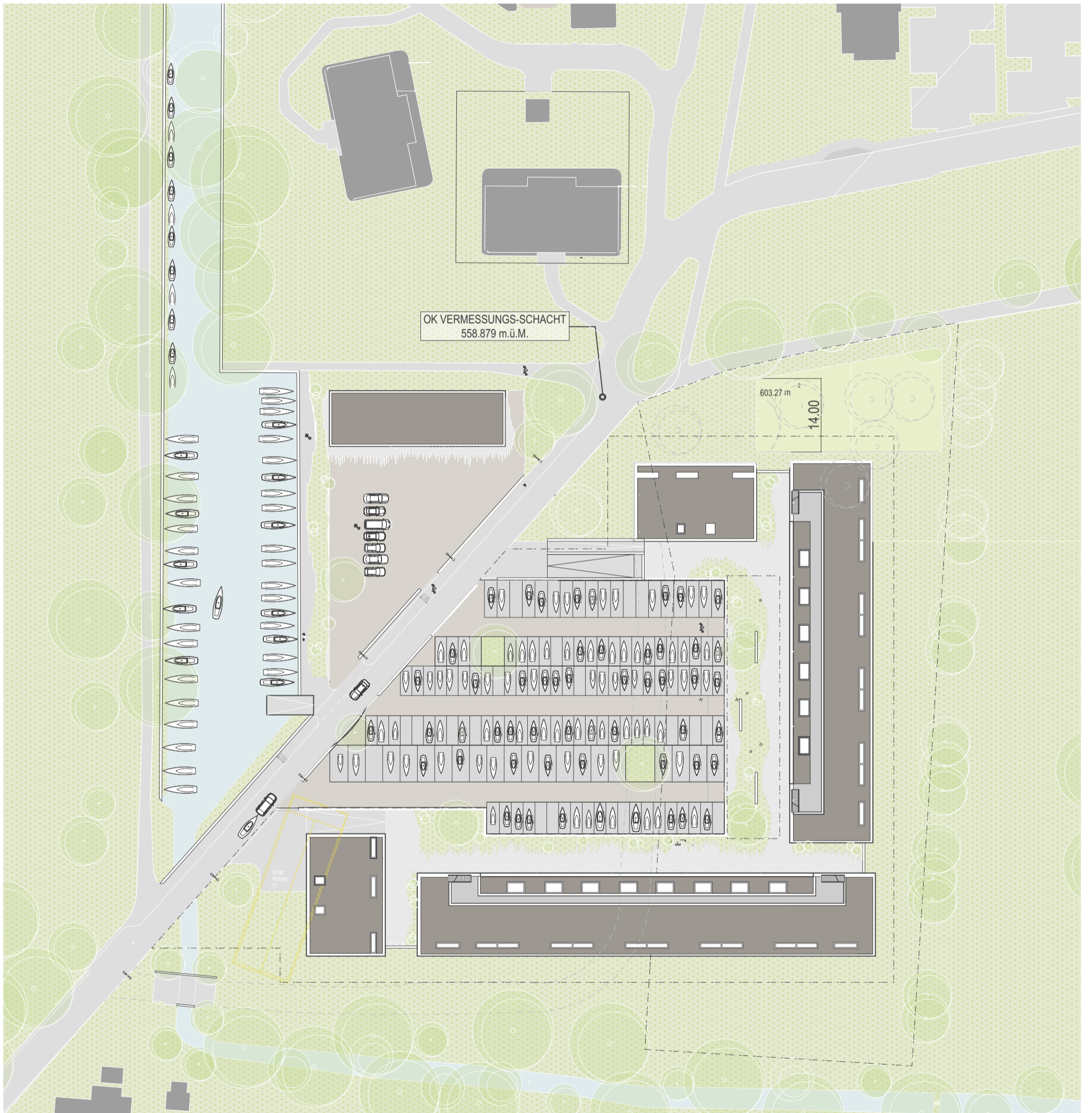
Situationsplan 1:750
